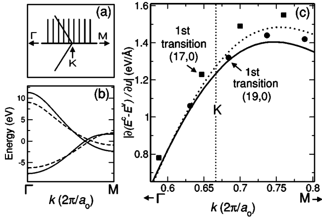
FIG. 2. (a) Detail of the Brillouin zone (BZ) of graphene around K with the band lines of a (19,0) nanotube and the \Gamma - K - M line. (b) Electronic bands of graphene along \Gamma - K - M in equilibrium (solid line) and under a deformation of 0.1 Å corresponding to the RBM of a (19,0) tube (dashed line, difference enhanced \times 10 ). (c) Calculated \partial E_b(\mathbf{k})/\partial \mathbf{u} for a (17,0) (squares) and a (19,0) (circles) tube, and of graphene deformed to simulate the RBM of a (19,0) tube (solid line) and a (17,0) nanotube (dotted line).
