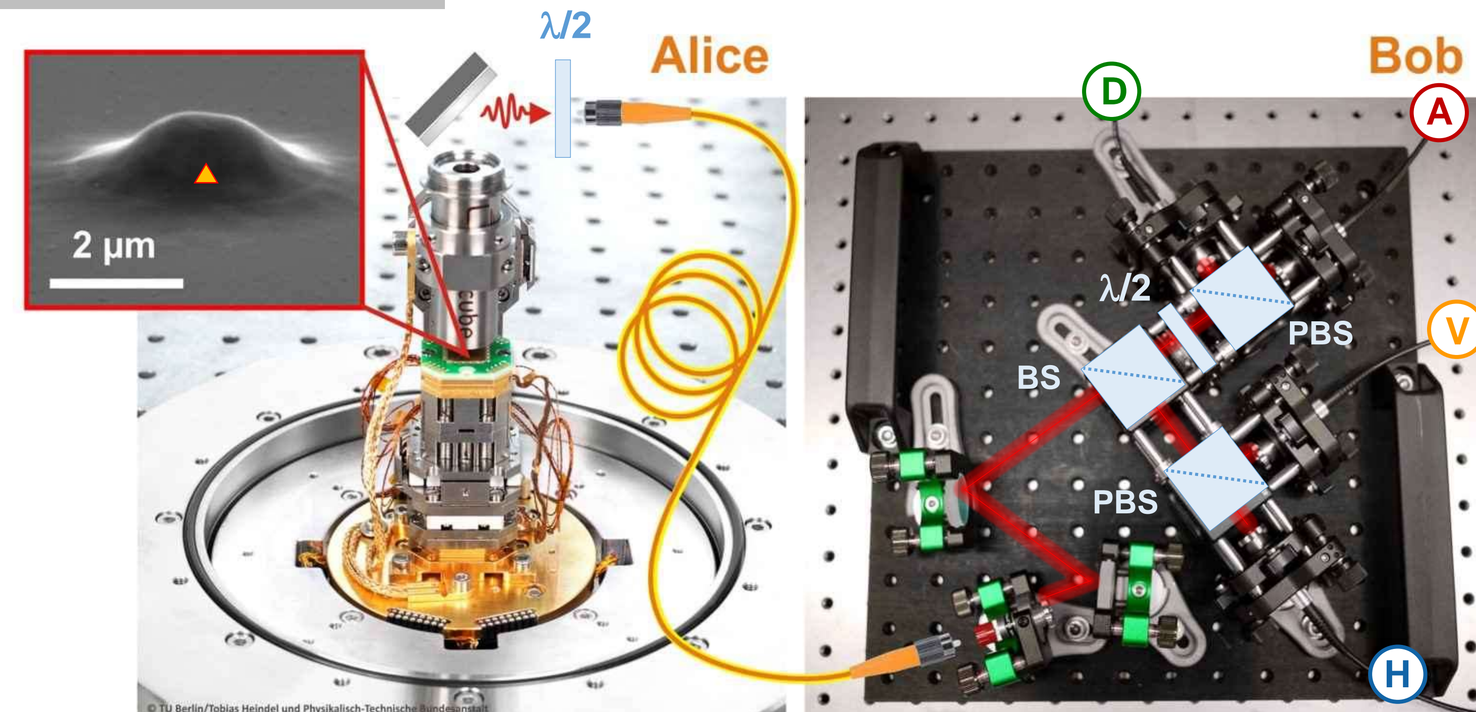
Deterministically fabricated QD single-photon source [1]
