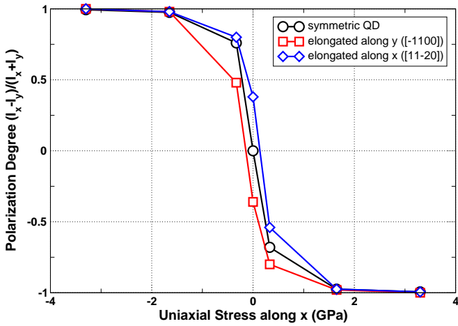
FIG. 9: (Color online) Polarization degree of the excitonic ground-state transition as a function of uniaxial stress along x ( [11\bar{2}0] ), relaxation of the sample in y and z direction according to the laws of continuum mechanics has been included. The calculations have been performed for three different QDs with an aspect ratio of h:d = 1:10 and a height of h = 2.0 nm. Black lines and circles : Symmetrical QD. Blue lines and diamonds : QDs with 10% elongation along x . Red line and squares : QDs with 10% elongation along y .
