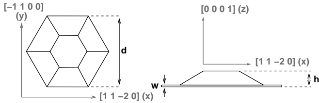
FIG. 4: Model structure of c -plane GaN/AlN QDs: Truncated hexagonal pyramid with height h between 1.5 nm and 3.5 nm. The lateral diameter d is determined by the dot's aspect ratio h:d = 1:10 (1:5). The wetting-layer thickness is w = 0.25 nm.
