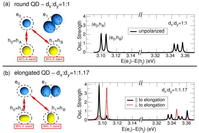
FIG. 2: (Color online) Confined single-particle electron (blue) and hole (yellow) states in a round (a) and an elongated (b) QD. The corresponding interband transitions are shown on the right-hand side. For the round QD, the A - and B -band transitions emit unpolarized light (with k \parallel C ), while the respective transitions in the elongated QD are polarized parallel and perpendicular to the long axis of the QD. The transitions between 3.33 and 3.36 eV originate from higher excited electron and hole levels.
