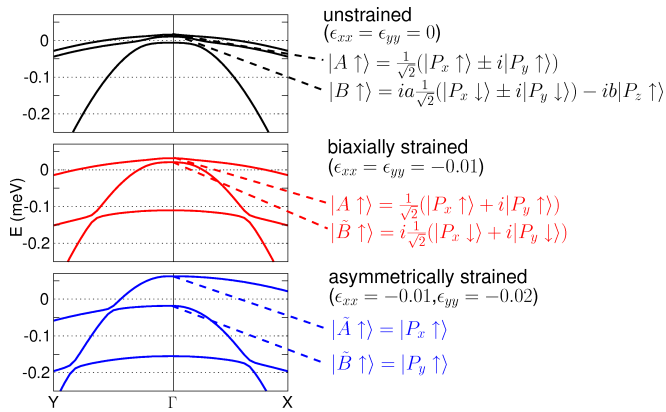
FIG. 7: (Color online) Valence band structure of GaN in the vicinity of \Gamma . Upper panel : unstrained. center : under symmetric biaxial strain in the basal plane, typical for c -plane QDs. Lower : With an additional strain anisotropy in the basal plane, e.g., in asymmetric QDs. The splitting between the two top bands increases and their characters change from A - and B -like to P_x -like and P_y -like.
