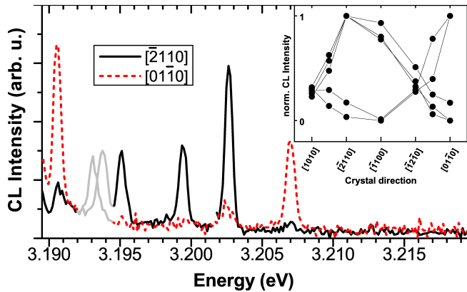
FIG. 1: (Color online) CL spectrum of a single InGaN/GaN QD. Grey lines belong to a different QD. The inset shows the evolution of the intensities of the five lines as a function of the polarization angle.
