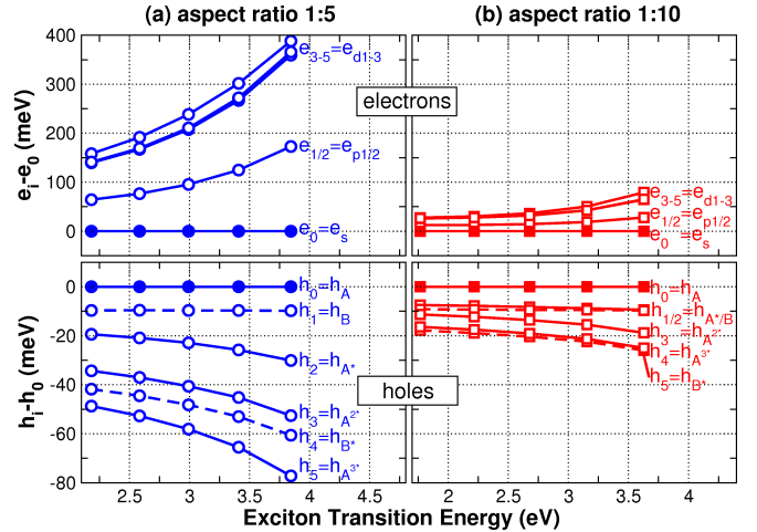
FIG. 6: (Color online) Energies of the single-particle electron and hole states. The electron states are labeled according to the symmetry of their envelope functions ( s , p , and d shell). Hole-state labels are given according to the valence band from which the hole states are predominantly formed.
