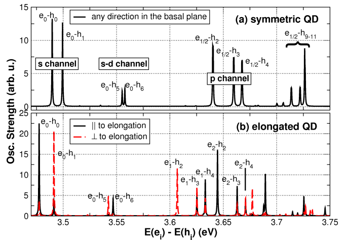
FIG. 8: (Color online) Oscillator strength between the single-particle electron and hole state for a QD with an aspect ratio of h:d = 1 : 5 and a height of h = 2.0 nm. Shown are all transitions involving one of the first six electron levels ( e_i ) and one of the first twelve hole levels ( h_j ), but only up to an energy difference e_i - h_j of 3.75 eV. (a) For a symmetric QD. (b) For a QD with a 10% in-plane elongation along [11\bar{2}0] .
