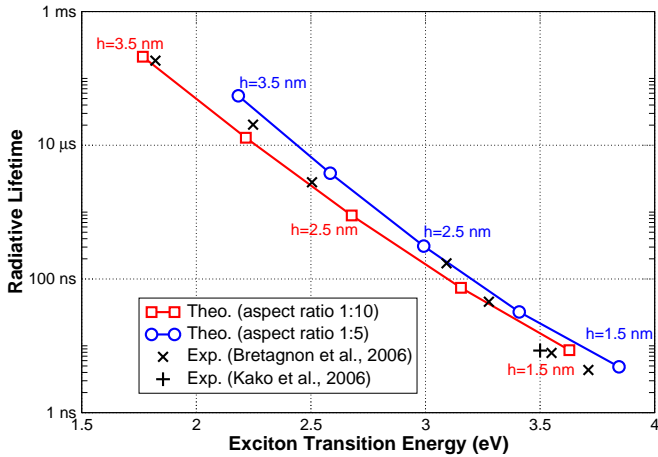
FIG. 5: (Color online) Radiative lifetimes of confined excitons in c -plane GaN/AlN QDs: Red lines and squares : Calculated, QDs with an aspect ratio of h:d = 1:10 . Blue line and circles : Calculated, QDs with an aspect ratio of h:d = 1:5 . Black crosses : Experimental values from Bretagnon et al. [29]. Black plus : Experimental value from Kako et al. [14].
