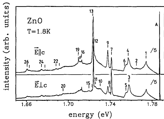
FIG. 1. Polarized luminescence spectra of a typical high-quality ZnO rod excited at 2.71 eV.
