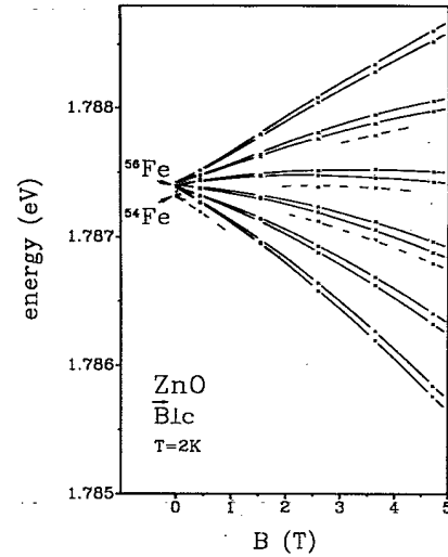
FIG. 5. Zeeman pattern of the zero-phonon region of the luminescence shown in Fig. 1, for the magnetic-field orientation B\perp c . Solid lines correspond to the dominating lines as shown in Fig. 3 attributed to ^{56}\text{Fe} in an \text{O}^{16} surrounding. Dashed lines correspond to lines shifted by an isotope effect of the iron ( ^{54}\text{Fe} ).
