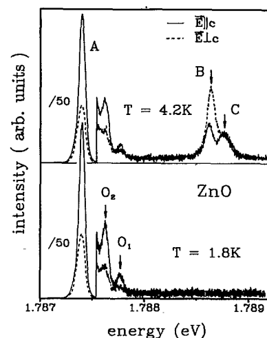
FIG. 15. Polarized luminescence spectra of the ZPL region at 1.8 and 4.2 K excited with the 2.71-eV line of an \text{Ar}^+ -ion laser. The weak lines marked by O_1 and O_2 are shifted with respect to the dominating ZPL A by the presence of one \text{O}^{18} ion in the \text{Fe}^{3+}\text{O}_4^{2-} cluster.
