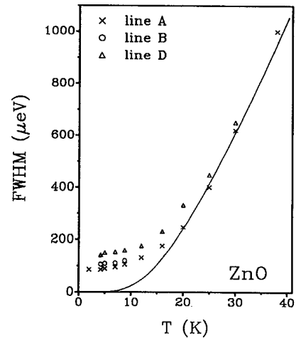
FIG. 7. Temperature dependence of the FWHM's of the ZPL's A, B, and D. The solid line gives a fit assuming the interaction of resonant low-frequency phonons with the electronic fine structure of the {}^4T_1(G) state.
