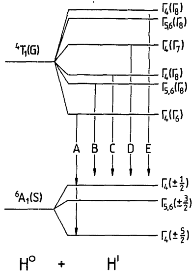
FIG. 13. Simplified term scheme of Fe 3+ . H^0 contains the interelectronic Coulomb interaction and the T_d crystal field, H^1 contains the spin-orbit interaction, the spin-spin interaction, the C_{3v} crystal field, and an intermediate Jahn-Teller interaction with E modes. The observed ZPL's are represented by arrows. The spacings are not given on a unique energy scale.
