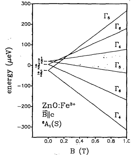
FIG. 12. Calculated fine structure of the {}^6A_1(S) state of isolated \text{Fe}^{3+} in ZnO in a magnetic field with \mathbf{B} \parallel c . The parameters used are taken from ESR results (Ref. 24).
