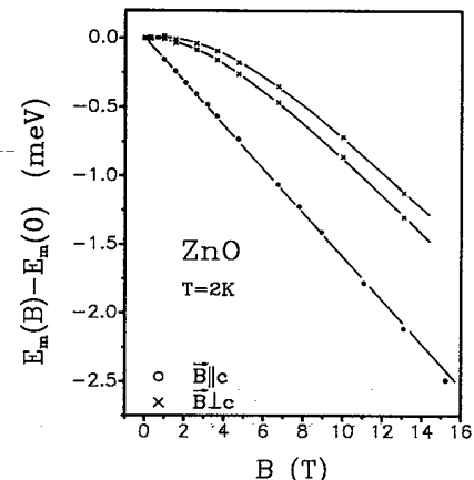
FIG. 8. Magnetic-field dependence of the lowest excited state in the orientations B||c and B⊥c. The center of gravity of the {}^6A_1(S) state is assumed to be independent of the magnetic field.
