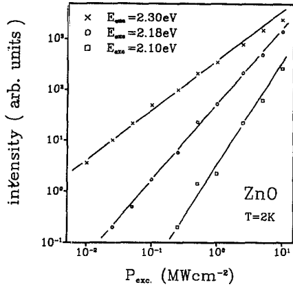
FIG. 11. Double logarithmic plot of the intensity of the luminescence shown in Fig. 1 with the excitation density for different excitation energies, using 15-ns pulse of an excimer laser-pumped dye laser.
