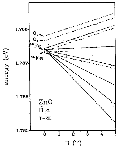
FIG. 4. Zeeman pattern of the zero-phonon region of the luminescence shown in Fig. 1, for the magnetic-field orientation B\parallel c . Solid lines correspond to the dominating lines as shown in Fig. 3 attributed to ^{56}\text{Fe} in an \text{O}^{16} surrounding. Dashed lines correspond to lines shifted by isotope effects, either of the iron ^{54}\text{Fe} or of the oxygen ( \text{O}_1, \text{O}_2 ) in the \text{Fe}^{3+}\text{O}^{2-}_4 cluster.
