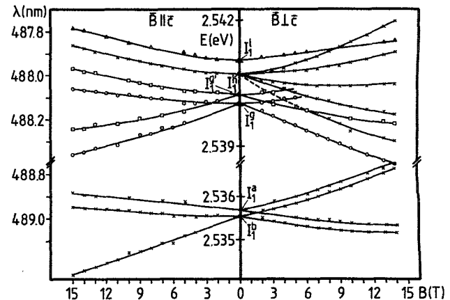
FIG. 4. Zeeman splitting of the lines I_1^{a,b} and I_1^g - I_1^l in a magnetic field in Voigt configuration k \parallel c .
