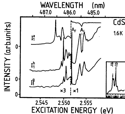
FIG. 5. Excitation spectra of I_1^a , I_1^q , and I_1^h (luminescence spectrum shown in the inset of the figure) under pulse laser light. For the description of the various excitation resonances, see text.
